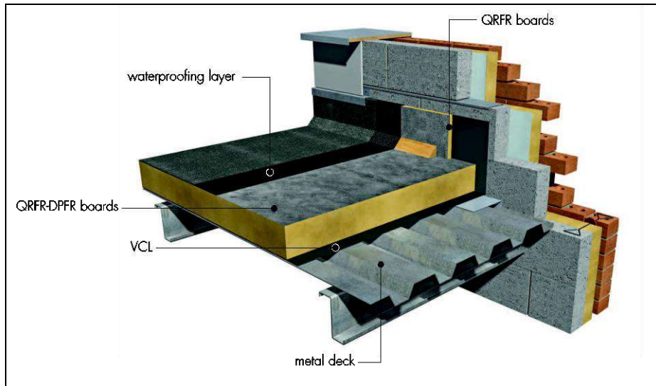
Figure 4 Installation — Metal deck
