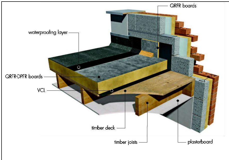
Figure 2 Installation — Timber deck
