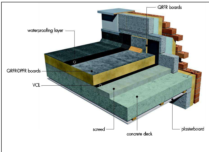
Figure 3 Installation — Concrete deck
